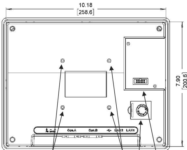
Rear View
